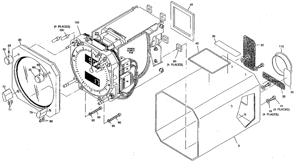
IPL FIGURE 1. MODEL 2610 ELECTRONIC CHRONOMETER, P/N 2610-08-1.
