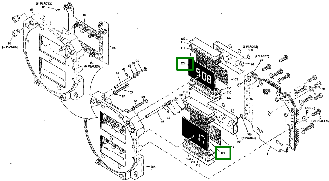
IPL FIGURE 8. DISPLAY ASSEMBLY, P/N 101067-01-01, -02-01.
